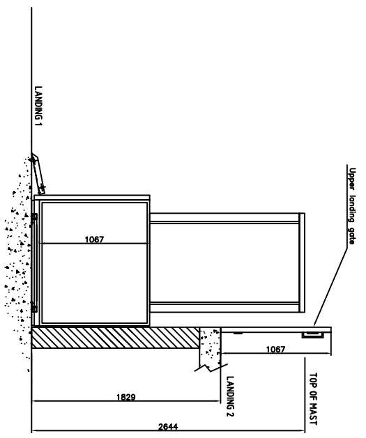
Side view for EleveX Typ 2
